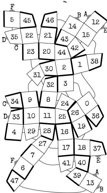
Joined Rhombicuboctahedron
