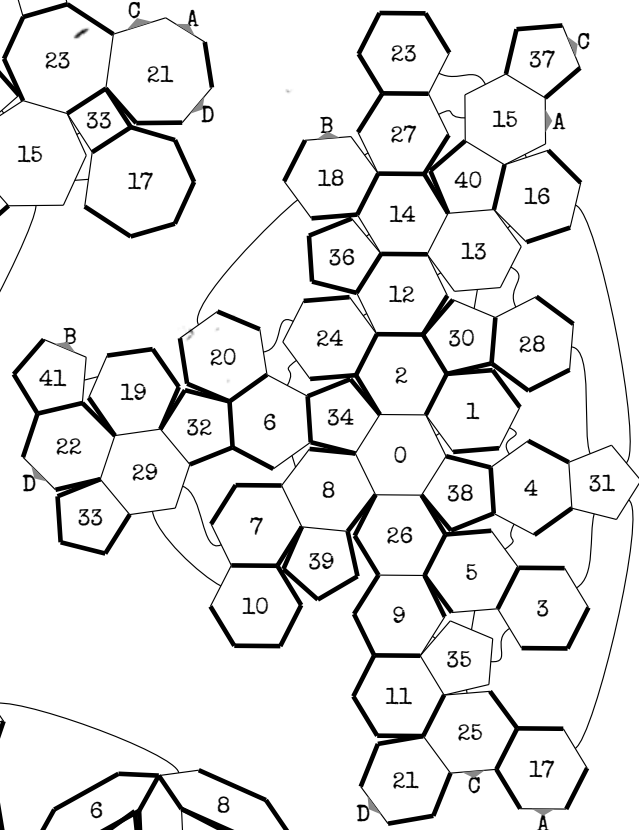
Chamfered Dodecahedron
