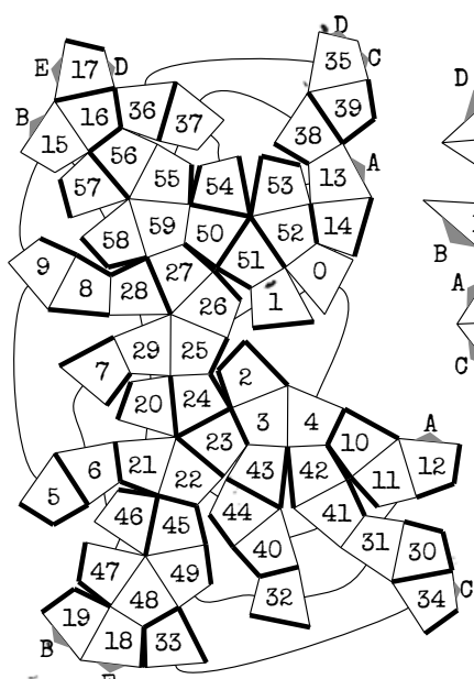
Deltoidal Hexecontahedron
